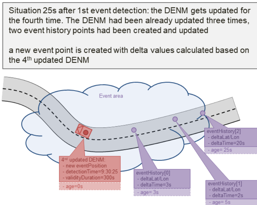
Figure 3 (h) - Generation and evolution of eventHistory along an event area
